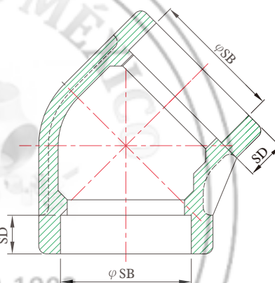
Socket-Weld End
